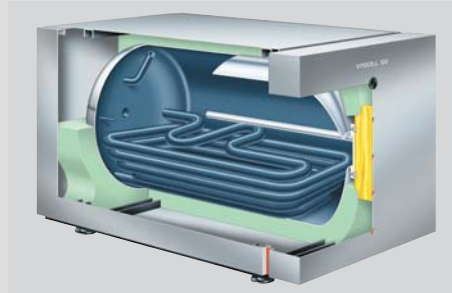
Vitocell-H 100 Space-saving design
