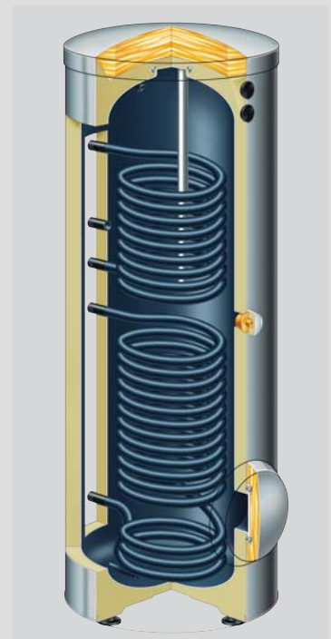
Vitocell-B 100 dual-coil solar tank
