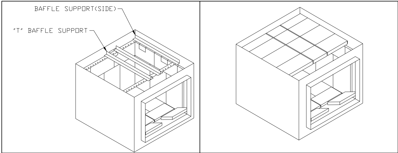
Figure 9 Ceramic Insulation Removed For Clarity
