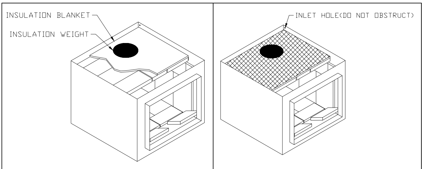
Figure 11 Cutaway Top View Of Stove
